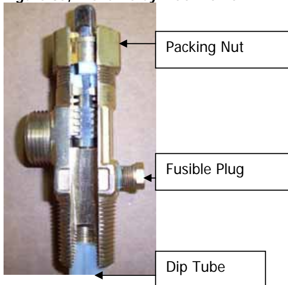
Figure 3a, ProFume Cylinder Valve
